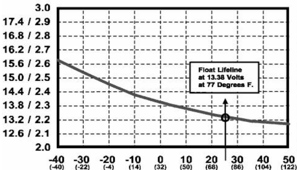
Figure 4. Optimum Charge Voltage versus Temperature
